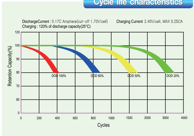
Cycle life characteristics
