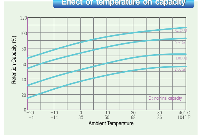
Effect of temperature on capacity
