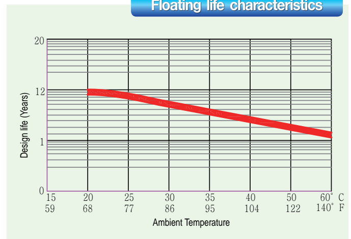
Floating life characteristics
